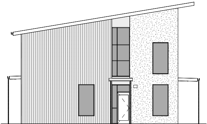
EAST ELEVATION
